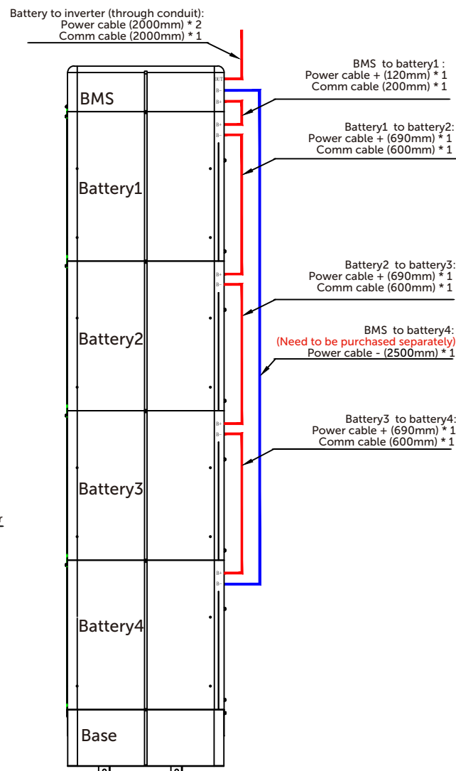
BMS * 1 & Battery * 4 wiring diagram ( I )
