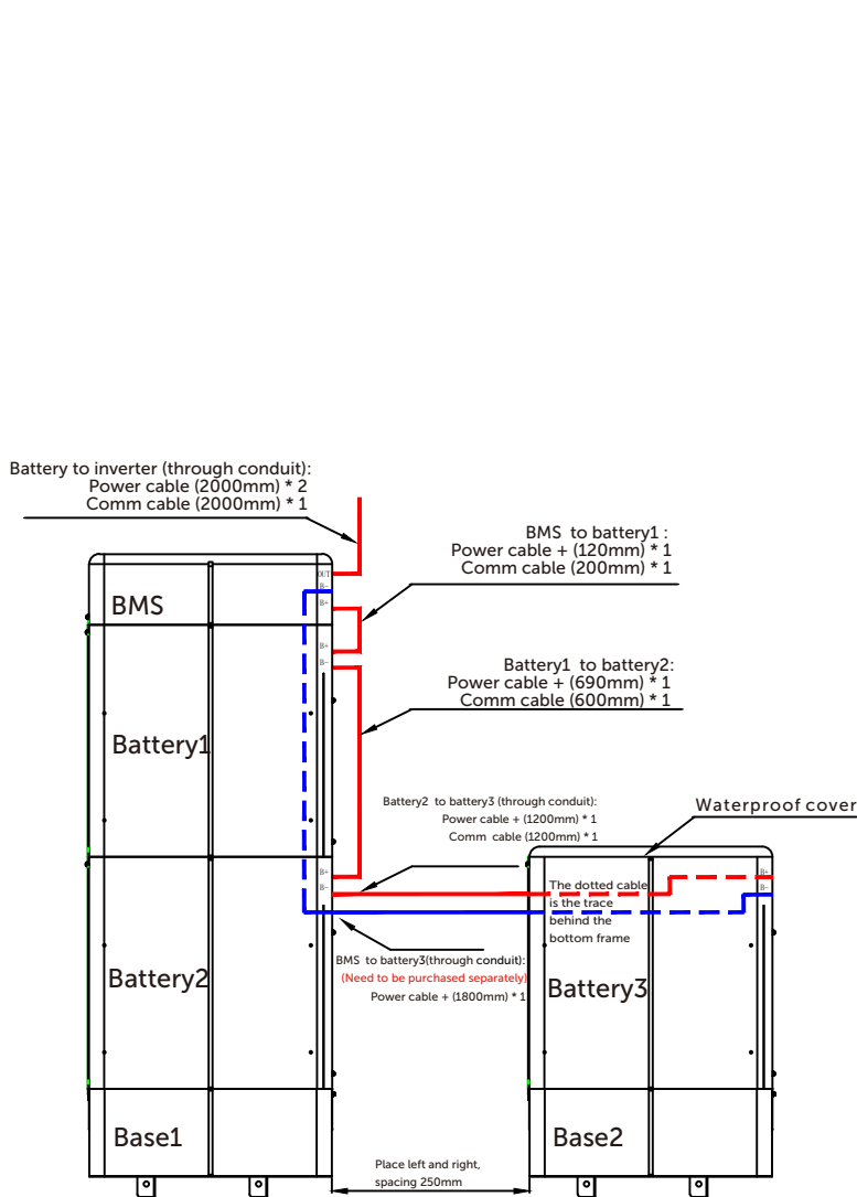
BMS * 1 & Battery * 3 wiring diagram ( II )
