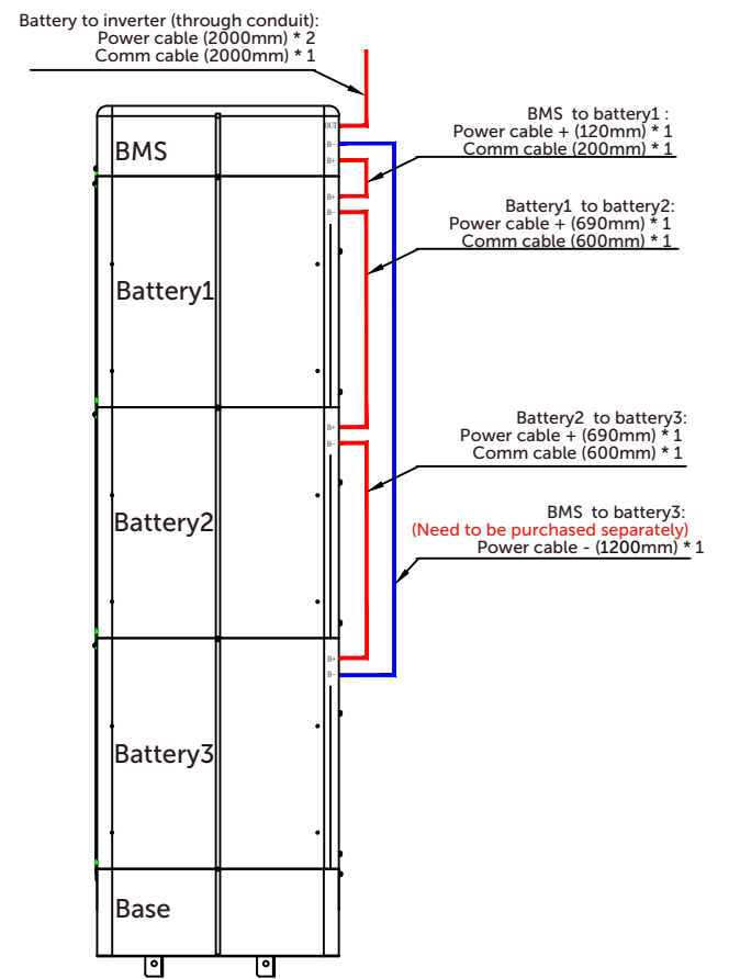
BMS * 1 & Battery * 3 wiring diagram ( I )
