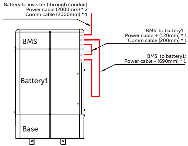
BMS * 1 & Battery * 1 wiring diagram
