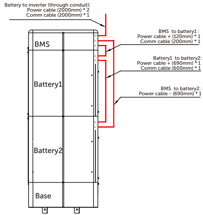
BMS * 1 & Battery * 2 wiring diagram
