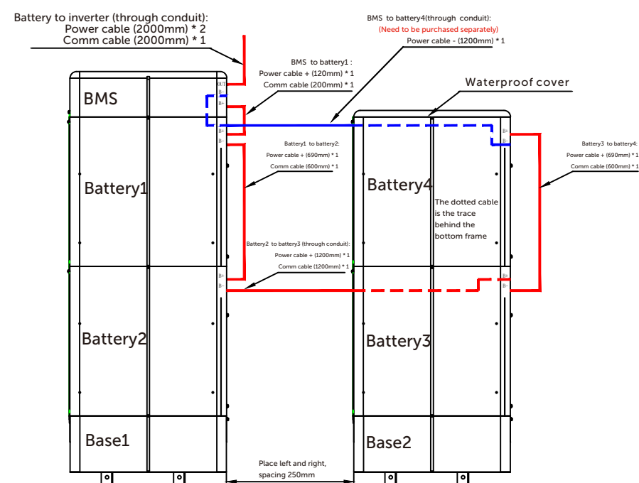
BMS * 1 & Battery * 4 wiring diagram ( II )
